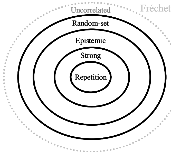
Figure 10: Categories of ‘independence’ for imprecise probabilities.
