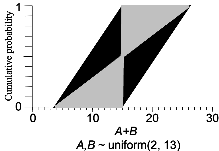
Figure 41. The range of distributions of sums A+B obtainable from Monte Carlo simulations varying the A, B correlation between -1 and +1 (gray cone) and best possible limits on these distributions making no assumptions about dependence (black parallelogram).
