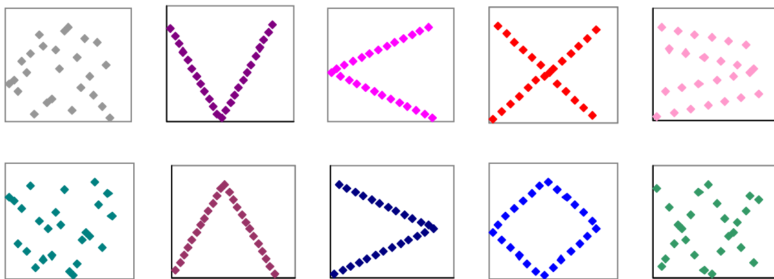
Figure 7: Some possible patterns of dependence between uncorrelated variables.
