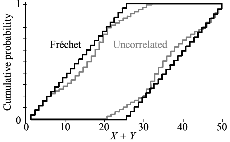
Figure 36: Bounds on convolution assuming inputs are uncorrelated compared to bounds under the Fréchet case for X, Y \sim \text{discreteuniform}(1,25)
